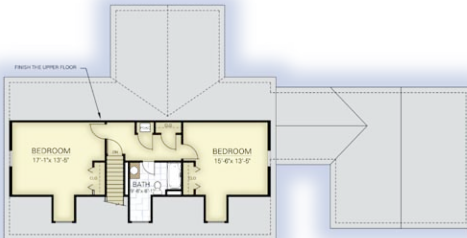
SECOND FLOOR PLAN 8' CEILING HEIGHT
