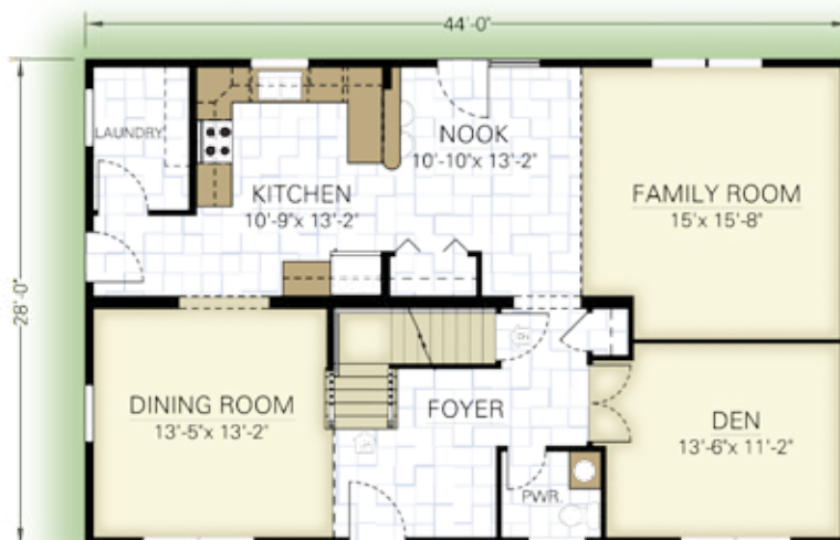
FIRST FLOOR PLAN * OPTIONAL FEATURES SHOWN
