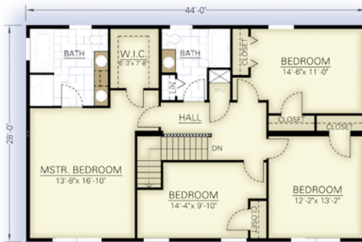
SECOND FLOOR PLAN * OPTIONAL FEATURES SHOWN
